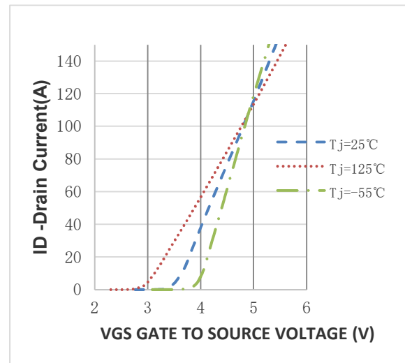
Figure 10. Transfer Characteristics
