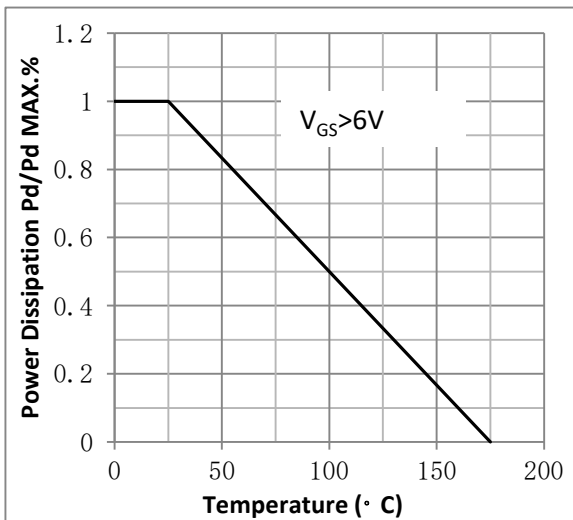
Fig.3 Power Dissipation
